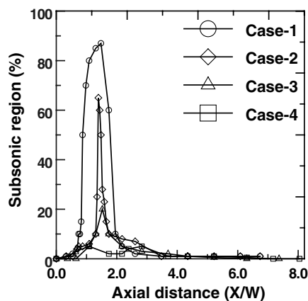
Fig. 5 Comparison of the subsonic region.
